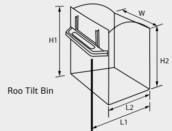
Roo Tilt Bin with Cabinet
