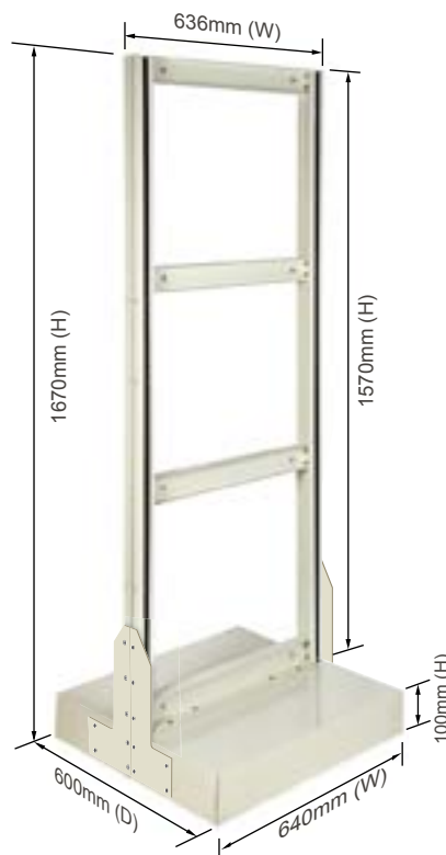
Double Sided Stand for Roo Tilt Bins Size: 640mm(W) x 1670mm(H) x 600mm(D)
