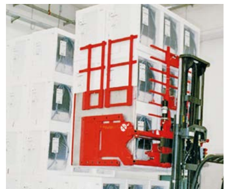
CARTON CLAMPS
